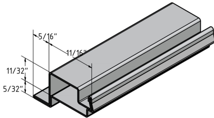
3/8" X 11/16" WITH STAGGERED FLANGE (.019, .021) SKU: FFS02 Category: Window Screen Bar UMO: FT
