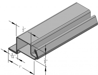
3/8" X 1" ROLLFORMED BAR W/LIP - - 13'6"
