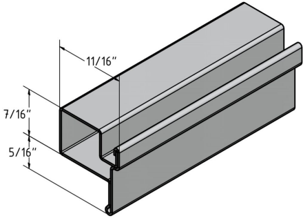
7/16" X 11/16" WITH LIFT (.024) SKU: FL01 Category: Window Screen Bar UMO: FT
