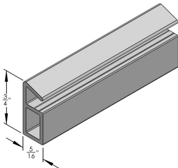
5/16" X 3/4" EXTRUDED BAR- 12' SKU: S-102 Category: Window Screen Bar UMO: FT
