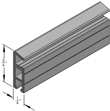
1/4" X 3/4" EXTRUDED BAR - 12' SKU: S-100 Category: Window Screen Bar UMO: FT
