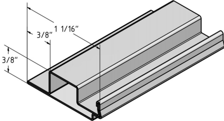
3/8" X 11/16" WITH REVERSE FLANGE (.019) SKU: FN02 Category: Window Screen Bar UMO: FT
