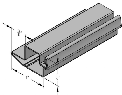
5/8 X 1/2" ROLLFORMED BAR W/ 3/8" LIP - 13'6"
