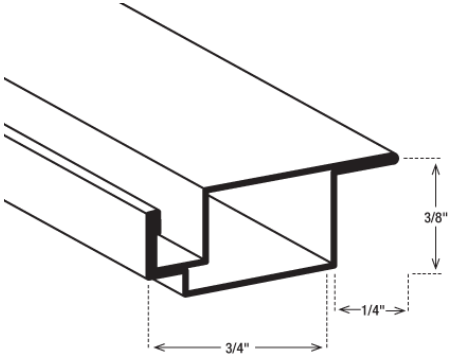
3/8" X 3/4" WITH 1/4" LIP SCREEN BAR (0.18, .021 GAUGE)--12'6"
