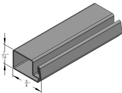
7/16" X 3/4" ROLLFORMED BAR - - 13'6"
