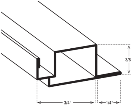
3/8" X 3/4" WITH 1/4" LIP ROLLFORMED BAR -- 12'6"
