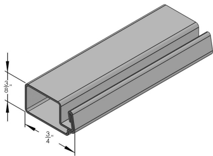
3/8" X 3/4" ROLLFORMED BAR - 13'6" SKU: S-125 (B38) Category: Window Screen Bar UMO: FT
