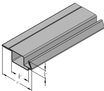
3/8" X 1" ROLLFORMED BAR W/LIP - 13'6"
