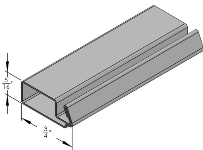
5/16" X 3/4" ROLLFORMED BAR - - 13'6"
