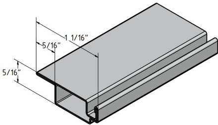
5/16" X 11/16" WITH LIFT (.019, .021) SKU: FF08 Category: Window Screen Bar UMO: FT
