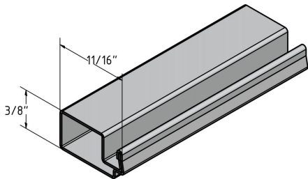
3/8" X 11/16" ROLLFORMED BAR - 12'6" (0.19", 0.24") SKU: FB02 Category: Window Screen Bar UMO: FT
