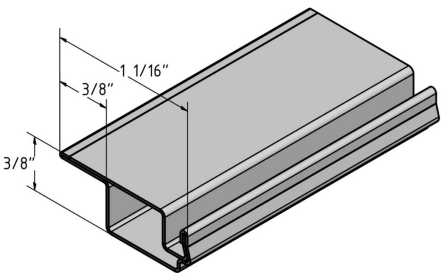
3/8" X 11/16" WITH FLANGE (.019, .024) SKU: FF02 Category: Window Screen Bar UMO: FT
