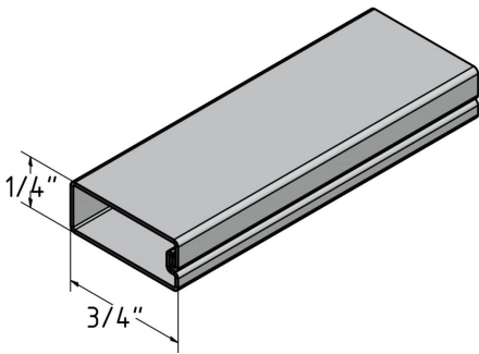
1/4" X 3/4" CROSSBRACE (.019) SKU: XB00 Category: Window Screen Bar UMO: FT
