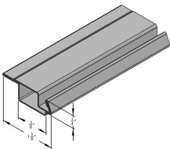
3/8" X 1 1/8" ROLLFORMED BAR W/LIP - 13'6"
