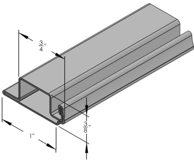
3/8" X 1" LIP ROLLFORMED BAR - 13'6"
