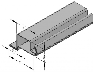
3/8" X 1" ROLLFORMED BAR W/LIP - - 13'6"
