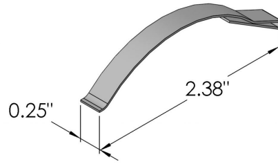
CORNER METAL COMPRESSION SPRING #9183 X .250 - STAINLESS STEEL
