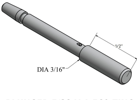
PLUNGER 5/32 X 1.560 ZINC
