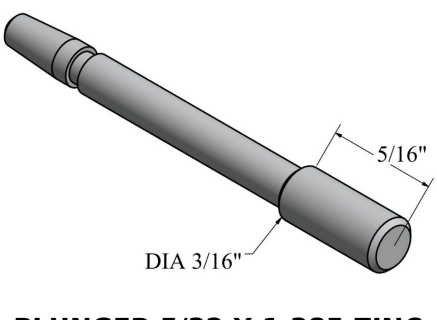
PLUNGER 5/32 X 1.385 ZINC
