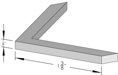
MITER CORNER FOR S-100 BAR - S-349 SKU: S-349 Category: Corners UMO: EA
