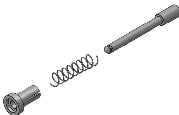
SPRING BOLT ASSEMBLY #138 - 1/8" NYLON WHITE
