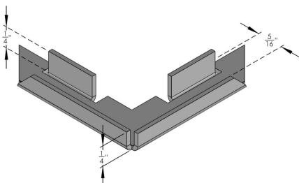
MITER CORNER FOR S-125,128,129 & 130 BAR
