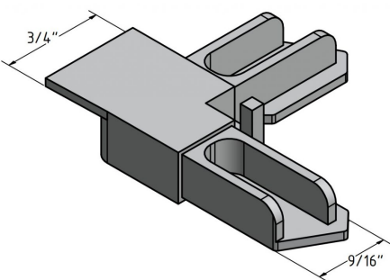
PLASTIC EXTERNAL RIGHT 1/2 FLANGE 3/8" FOR FF02 WITH FB02 BAR
