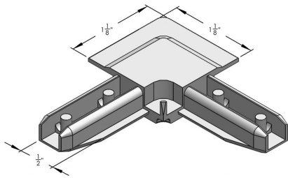
POLY CORNER FOR S-129 BAR SKU: S-356P Category: Corners UMO: EA
