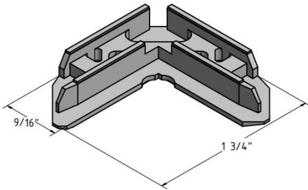
PLASTIC INTERNAL MITERED CORNER 7/16" FOR FB01, FL01 BAR
