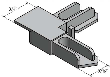
PLASTIC EXTERNAL LEFT 1/2 FLANGE 3/8" FOR FF02 WITH FB02 BAR
