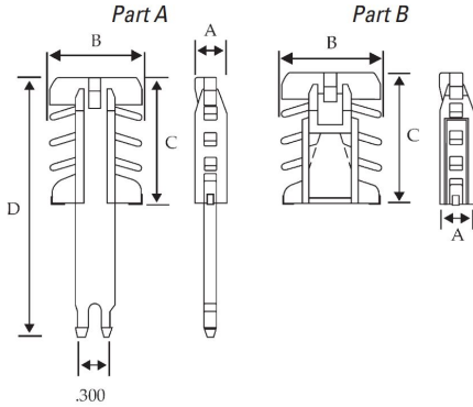
FISHMOUTH CONNECTOR SET 5.5X18MM SKU: S-539AB Category: Grille Bar Accessories UMO: EA
