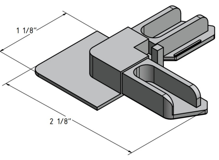
FLANGED POLY CORNER 3/8"FOR FF02 BAR
