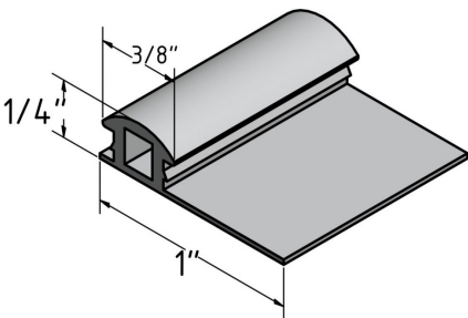
BUG FLAP - BLACK 1"
