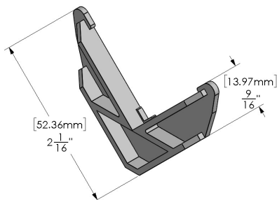
PLASTIC INTERNAL MITERED CORNER 5/16" FOR FB08, FF08, FL08
