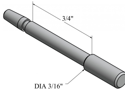
PLUNGER 5/32 X 1.445 ZINC
