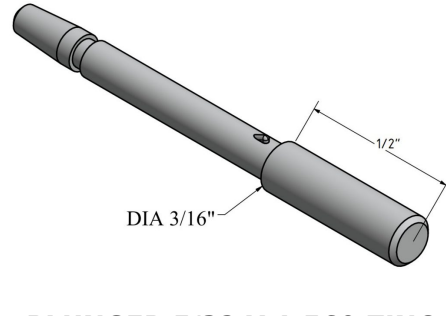
PLUNGER 5/32 X 1.560 ZINC
