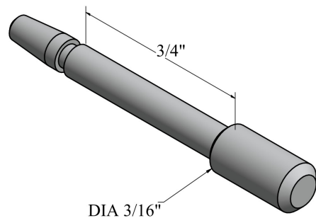
PLUNGER 3/16 X 1.387 ZINC*OB1
