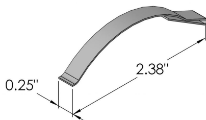
CORNER METAL COMPRESSION SPRING #9183 X .250 - STAINLESS STEEL
