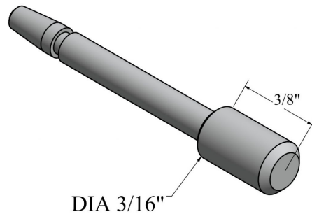
PLUNGER 7/32 X 1.433 ZINC
