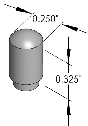
FIXED PIN
