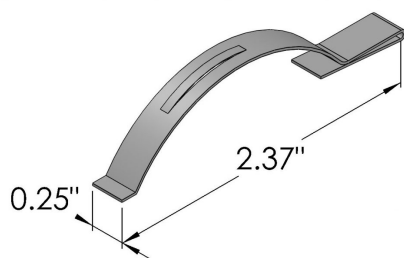
COMPRESSION SPRING (CORNER) WITH RETAINER CLIP - STAINLESS STEEL
