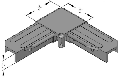
POLY CORNER FOR S-124 BAR
