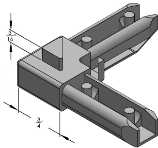
POLY CORNER FOR S-124 W/STOP OFF SKU: S-352P-STOP Category: Corners UMO: EA
