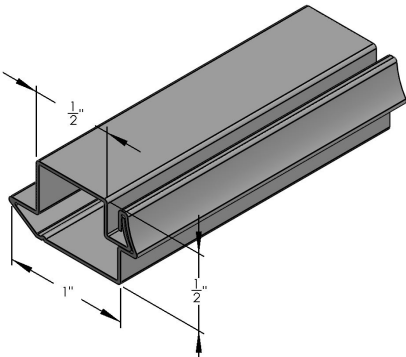
3/4" X 1/2" ROLLFORMED BAR W/ LIP - - 13'6"
