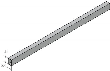
5/16" X 1/2" CROSSBRACE BAR - 13'
