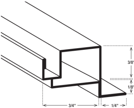
3/8" X 3/4" WITH STAGGERED 1/4" LIP ROLLFORMED SCREEN BAR -- 12'6" (0.18, 0.21 GAUGE)
