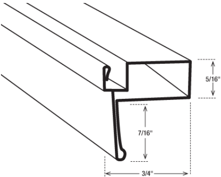
3/4" X 5/16" LIFT RAIL ROLLFORMED BAR
