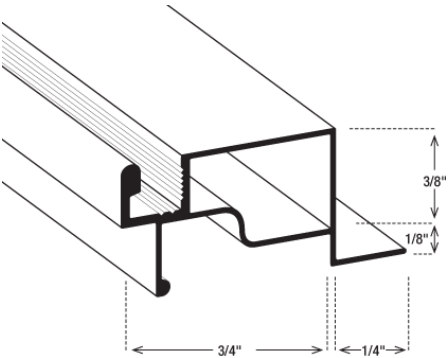
ALUMINUM BAR B9 EXTRUDED -
