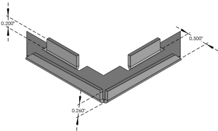
MITER CORNER FOR S-124 BAR
