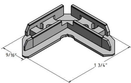
PLASTIC INTERNAL MITERED CORNER 7/16" FOR FB01, FL01 BAR
