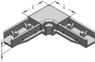
POLY CORNER FOR S-124 (1 3/4" BREAKDOWN) SKU: S-360P Category: Corners UMO: EA
