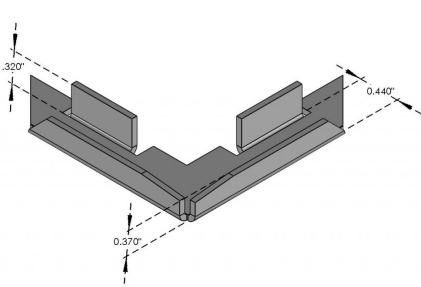
MITER CORNER FOR S-126 BAR SKU: S-350 Category: Corners UMO: EA
