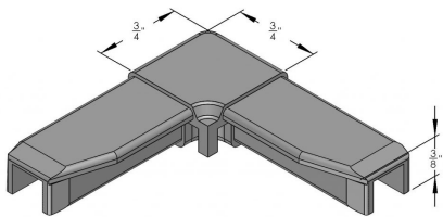
POLY CORNER FOR S-125 BAR SKU: S-351P Category: Corners UMO: EA
