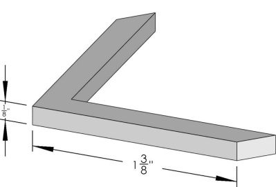
MITER CORNER FOR S-100 BAR - S-349 SKU: S-349 Category: Corners UMO: EA
