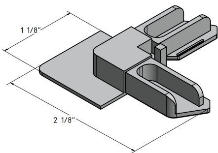
FLANGED POLY CORNER 3/8"FOR FF02 BAR
