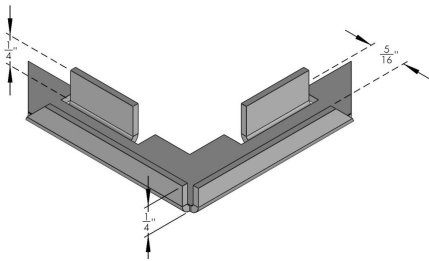
MITER CORNER FOR S-125,128,129 & 130 BAR SKU: S-351 Category: Corners UMO: EA
