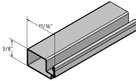
3/8" X 11/16" ROLLFORMED BAR - 12'6" (0.19", 0.24")
