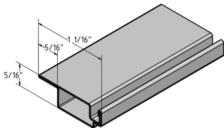
5/16" X 11/16" WITH LIFT (.019, .021)
