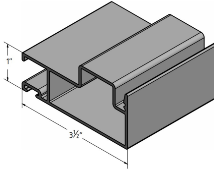
164" NPX .035 WP
