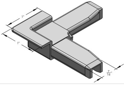
POLY CORNER FOR S-130 (1 3/4" BREAKDOWN)
