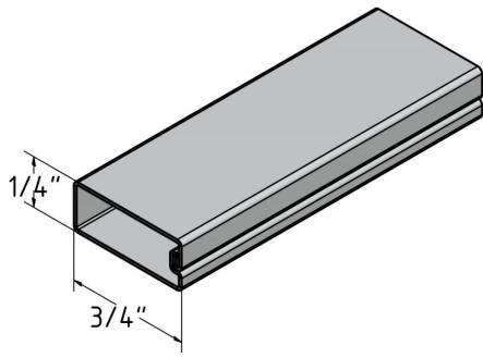
1/4" X 3/4" CROSSBRACE (.019)
