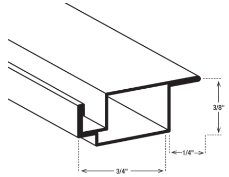
3/8" X 3/4" WITH 1/4" LIP SCREEN BAR (0.18, .021 GAUGE)--12'6"
