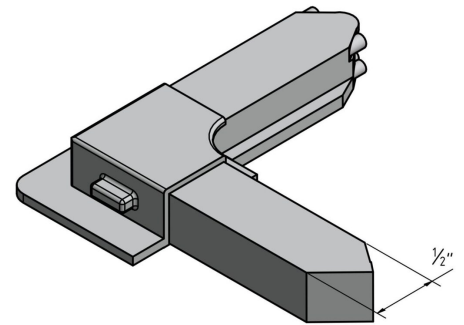
PLASTIC CORNER WITH BUMP FIXED RIGHT FOR B8A BAR
