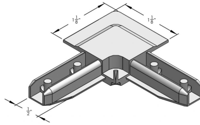
POLY CORNER FOR S-129 BAR
