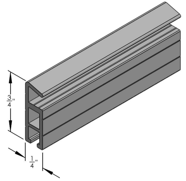
1/4" X 3/4" EXTRUDED BAR - 12'
