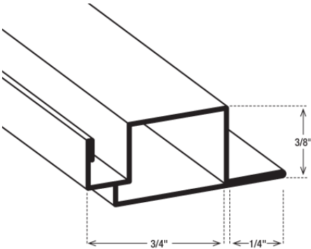
3/8" X 3/4" WITH 1/4" LIP ROLLFORMED BAR -- 12'6"
