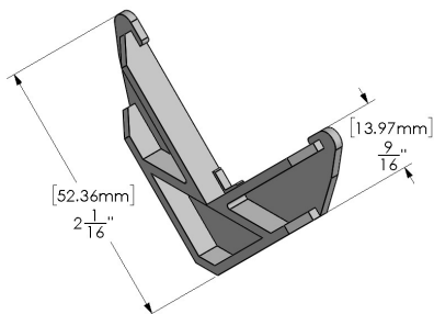
PLASTIC INTERNAL MITERED CORNER 5/16" FOR FB08, FF08, FL08
