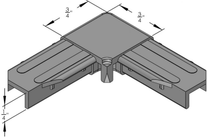
POLY CORNER FOR S-124 BAR SKU: S-352P Category: Corners UMO: EA
