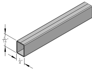
1/4" X 5/16" GRILLE BAR - 13'6" OR 12'8" SKU: S-121 Category: Grille Bar UMO: FT
