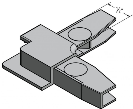
PLASTIC TAB CORNER WITH LIP RIGHT FOR B8B BAR
