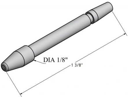
PLUNGER 5/32 X 1.345 ZINC SKU: HPL96-Plgr-Zinc Category: Window Screen Accessories UMO: EA
