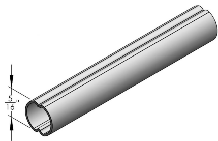
5/16" ROUND PENCIL MUNTIN - 12'8" SKU: S-131 Category: Grille Bar UMO: FT
