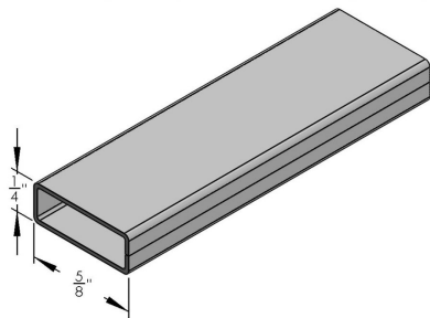
1/4" X 5/8" GRILLE BAR - 0.18 - 13'6" OR 12'8" SKU: S-120 Category: Grille Bar UMO: FT
