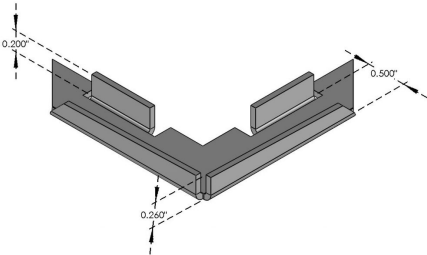
MITER CORNER FOR S-124 BAR SKU: S-352 Category: Corners UMO: EA
