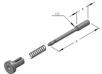
3/16" DIAMETER SPRING BOLT ASSEMBLY - PLASTIC HEAD - BLACK/WHITE
