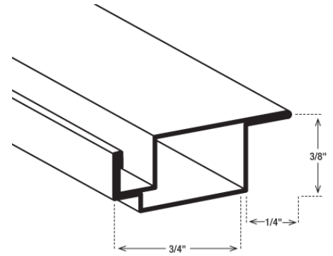
3/8" X 3/4" WITH 1/4" LIP SCREEN BAR (0.18, .021 GAUGE)--12'6"
