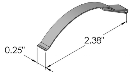
CORNER METAL COMPRESSION SPRING #9183 X .250 - STAINLESS STEEL
