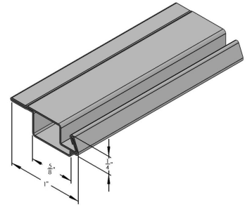
3/8" X 1" ROLLFORMED BAR W/LIP - 13'6"
