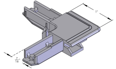
TABBED POLY CORNER FOR S-129S BAR LEFT/RIGHT
