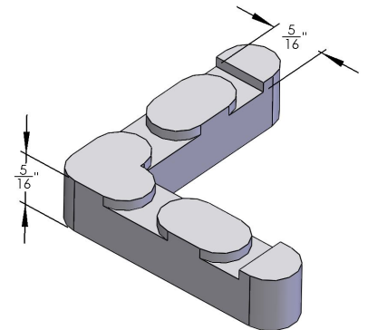
MITER CORNER FOR S-119 BAR
