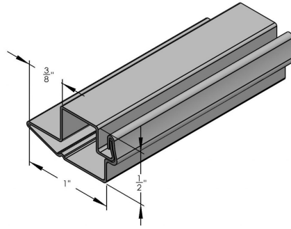
5/8 X 1/2" ROLLFORMED BAR W/ 3/8" LIP - 13'6"
