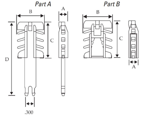
FISHMOUTH CONNECTOR SET 5.5X18MM SKU: S-539AB Category: Grille Bar Accessories UMO:EA
