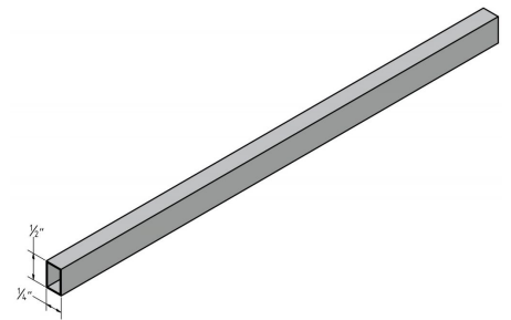
5/16" X 1/2" CROSSBRACE BAR - 13'
