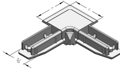
POLY CORNER FOR S-129S BAR
