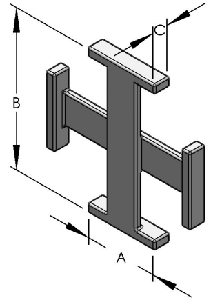
INTERNAL CROSS CONNECTOR FOR GRILLE 1/4" X 5/8" SKU: S-510 Category: Grille Bar Accessories UMO:EA
