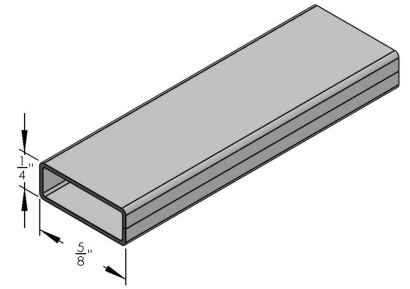
1/4" X 5/8" GRILLE BAR - 0.18 - 13'6" OR 12'8"
