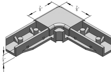
POLY CORNER FOR S-124 (1 3/4" BREAKDOWN)
