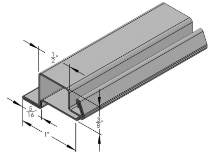
3/8" X 1" ROLLFORMED BAR W/LIP - - 13'6"
