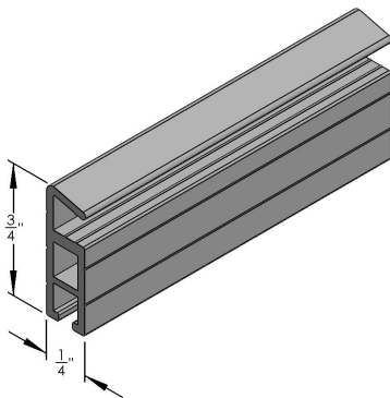
1/4" X 3/4" EXTRUDED BAR - 12'
