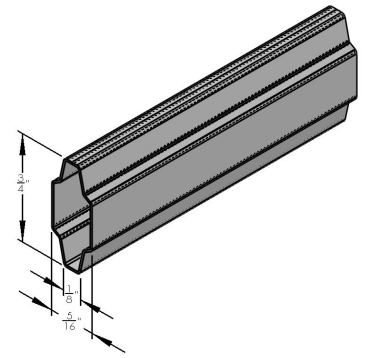
8MM X 18 MM GEORGIAN GRILLE BAR - 12'8"
