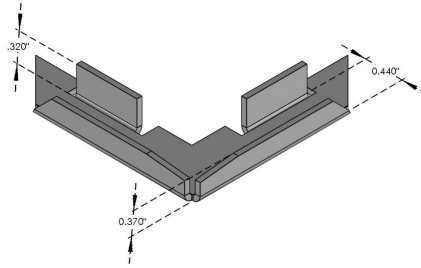
MITER CORNER FOR S-126 BAR
