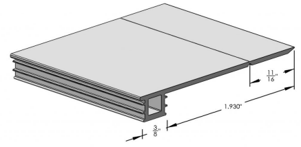
BUG STRIP VINYL - BLACK 2" 250FT
