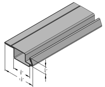
3/8" X 1 1/8" ROLLFORMED BAR W/LIP - 13'6"
