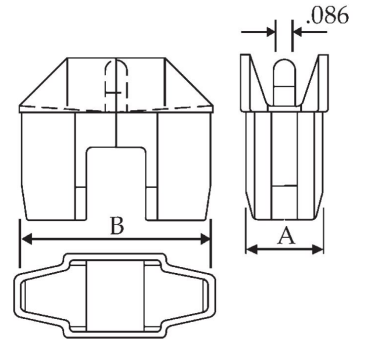
SADDLE CLIP FOR CONTOUR GRILLE 5.5X18MM
