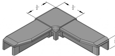
POLY CORNER FOR S-125 BAR
