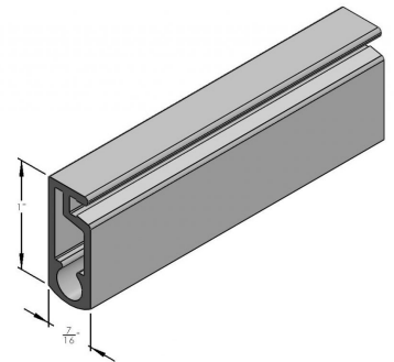
7/16" X 1" EXTRUDED BAR - 15.5'
