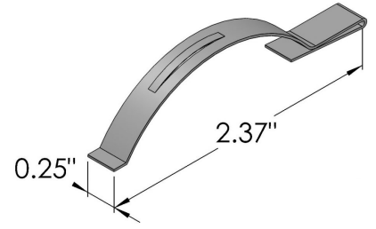
COMPRESSION SPRING (CORNER) WITH RETAINER CLIP - STAINLESS STEEL
