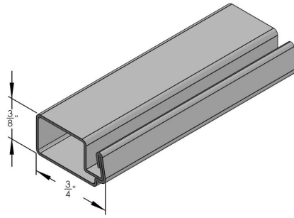
3/8" X 3/4" ROLLFORMED BAR - 13'6"
