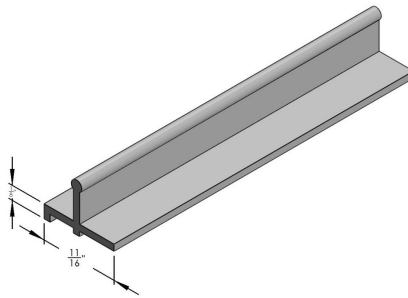
ALUMINUM SILL TRACK 12' (MILL)
