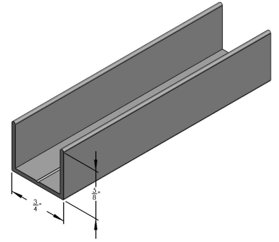
ALUMINUM JAMB TRACK (MILL, WHITE) --14 FT.
