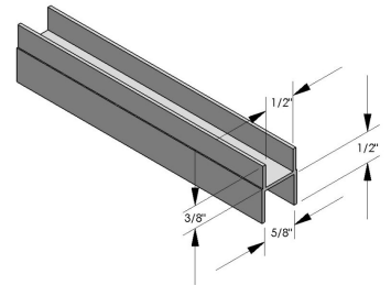
ALUMINIUM H JOINER 160" (MILL, WHITE)
