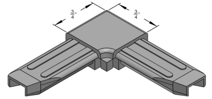
POLY CORNER FOR S-126 BAR - (S-350P)
