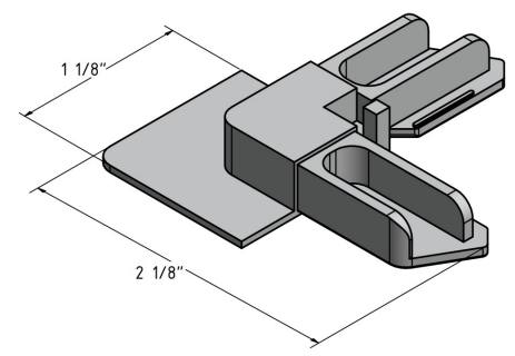
FLANGED POLY CORNER 3/8"FOR FF02 BAR
