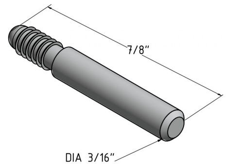
GRY NYL FIXED PIN 1 1/16"
