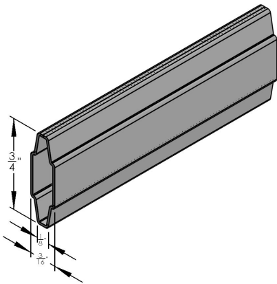
8MM X 25MM CONTOUR GRILLE BAR -- 152"
