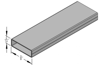
3/16" X 5/8" GRILLE - 152" LONG
