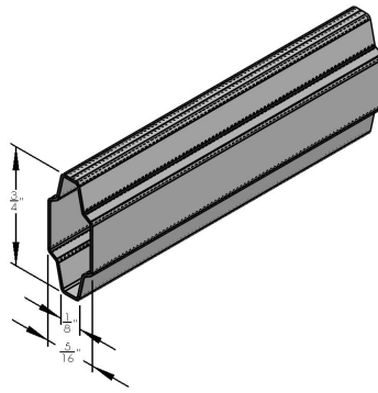
8MM X 18 MM GEORGIAN GRILLE BAR - 12'8"
