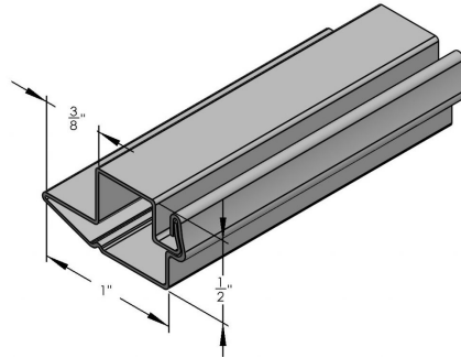
5/8 X 1/2" ROLLFORMED BAR W/ 3/8" LIP - 13'6" SKU: S-139 Category: Window Screen Bar UMO: FT
