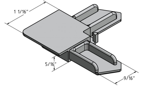
FLANGED POLY CORNER 5/16" FOR FF08 BAR
