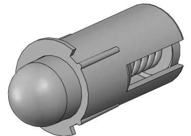
PLASTIC SPRING BUTTON BULLET CATCH
