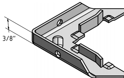
INT CORNER ALUM 3/8" FOR FB02, FF02, FFS02, FN02 BAR
