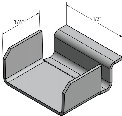
CROSSBAR INSERT INCB7-1
