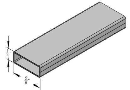
1/4" X 5/8" GRILLE BAR - 0.18 - 13'6" OR 12'8" SKU: S-120 Category: Grille Bar UMO: FT
