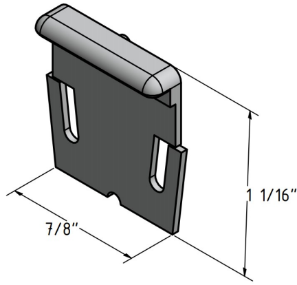
BGE .043 SLD LATCH 1025 SKU: HLA08 Category: Window Screen Accessories UMO: EA
