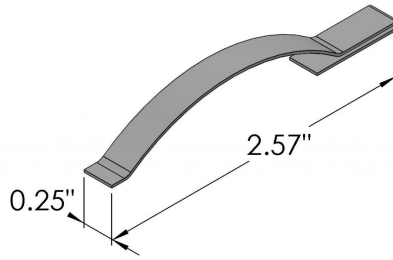
CORNER METAL COMPRESSION SPRING - STAINLESS STEEL
