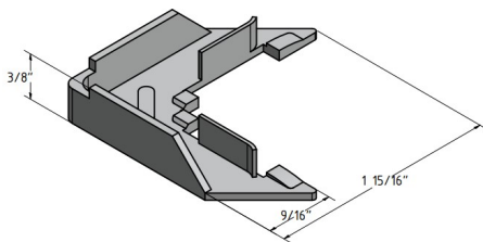
INT CORNER ALUM 7/16" FOR FB01, FL01
