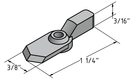
NAT SWIVEL LATCH
